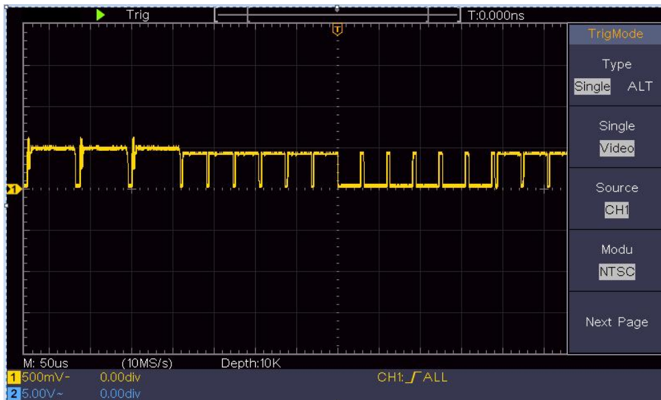
Figure 7-7 Waveform Captured from Video Field Trigger
